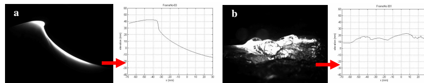
Figure 3. Examples of surface profile detection at breakpoint (a) and within the surf zone (b)
