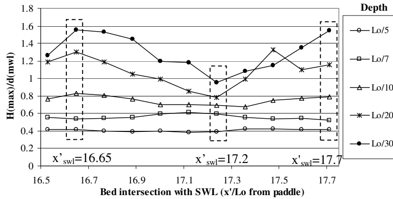
Figure 6. Evolution of the H_{max}/d_{mwl} ratio as a function of depth and group phasing
